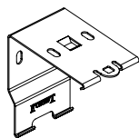
Support universel Easy plafond/face blanc BCS
